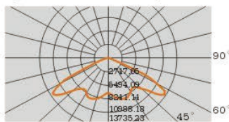
Light Distribution Curve C0/C180
